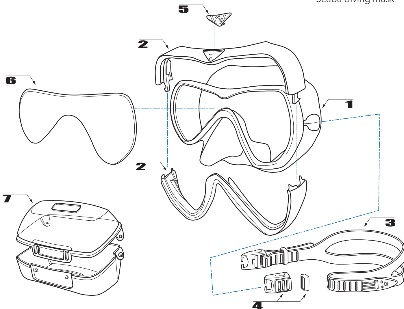
Product exploded view
